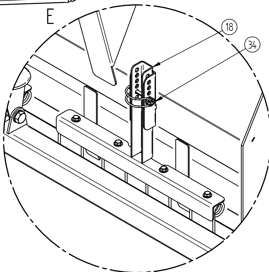
DETAIL E
