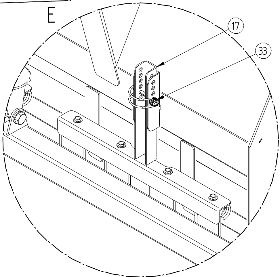
DETAIL E
