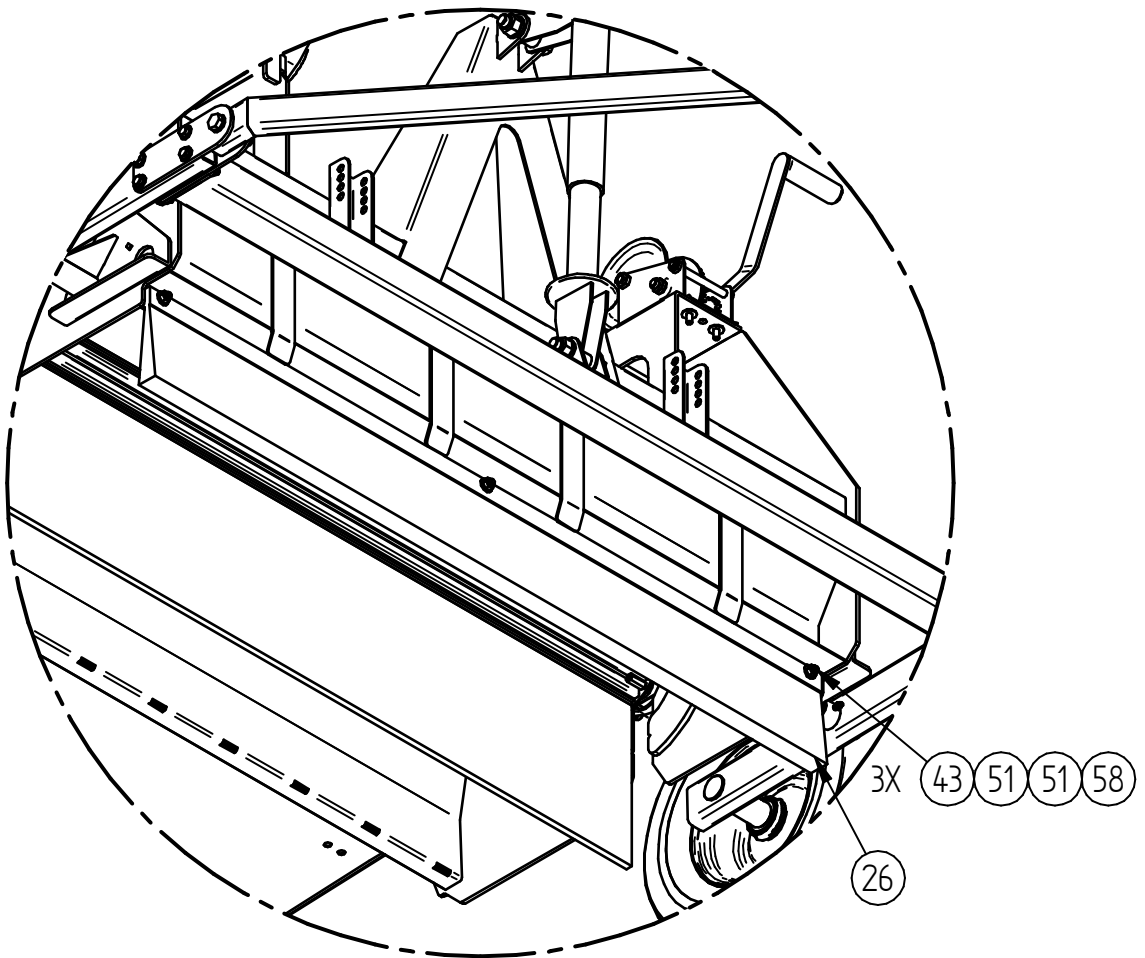
DETAIL C
