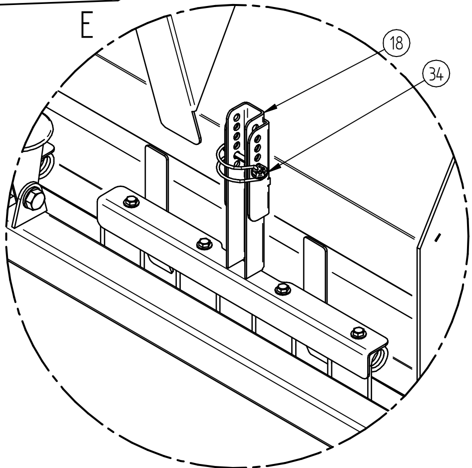
DETAIL E
