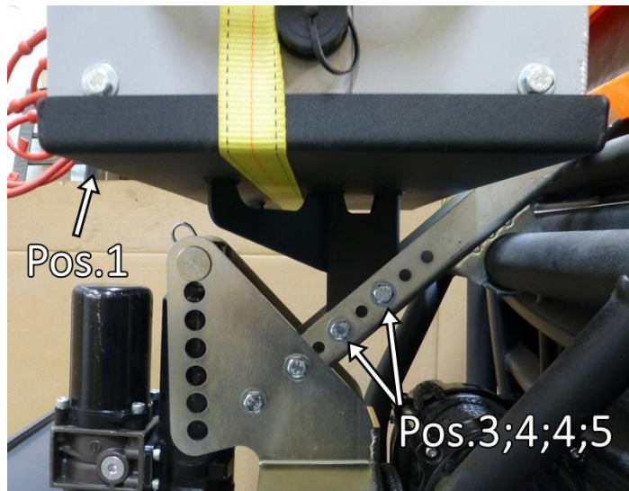
Paigaldus 71.10900 silindri hoidjaga
