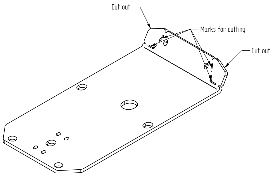
Iron Baltic skid plate front part
