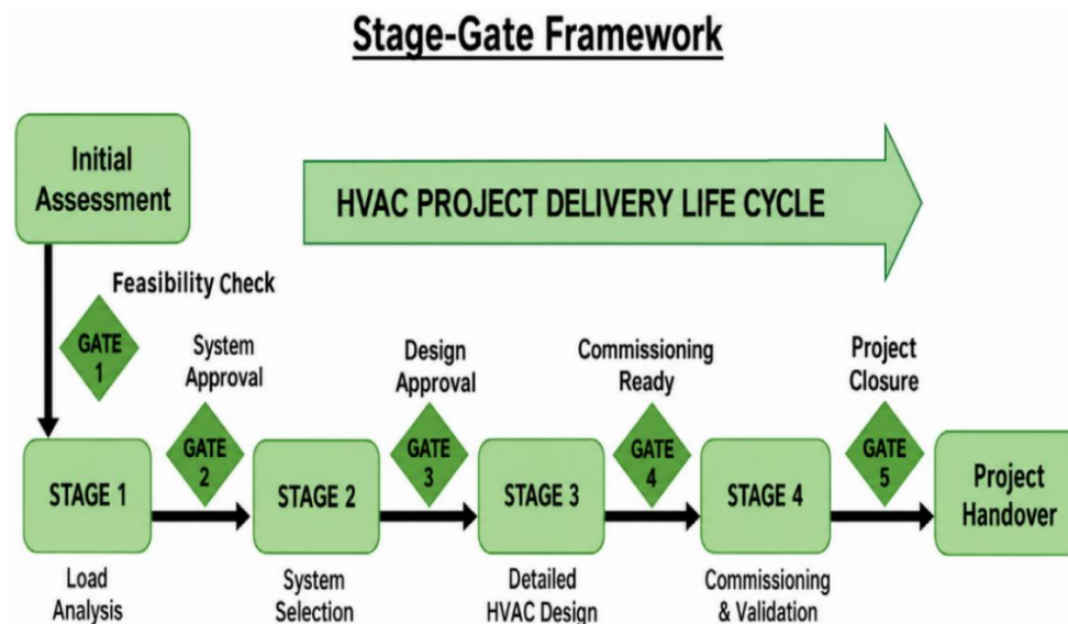
Fig. 2: Simplified life cycle representation of the stage-gated HVAC delivery and performance assurance framework.
