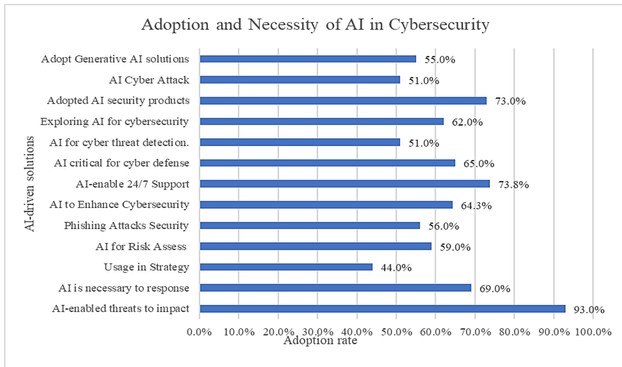
Fig. 7: Adoption and necessity of AI in cybersecurity.
