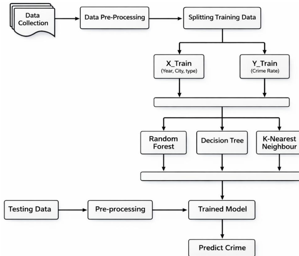
Fig. 1: System architecture.
