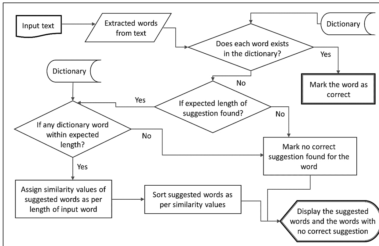
Fig. 1: Flowchart of the Konkani spell checker.
