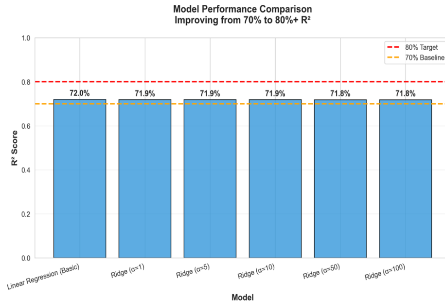
Fig. 2: Comparison of model performance across different regularization strengths, showing minimal variation in test R^2 values.
