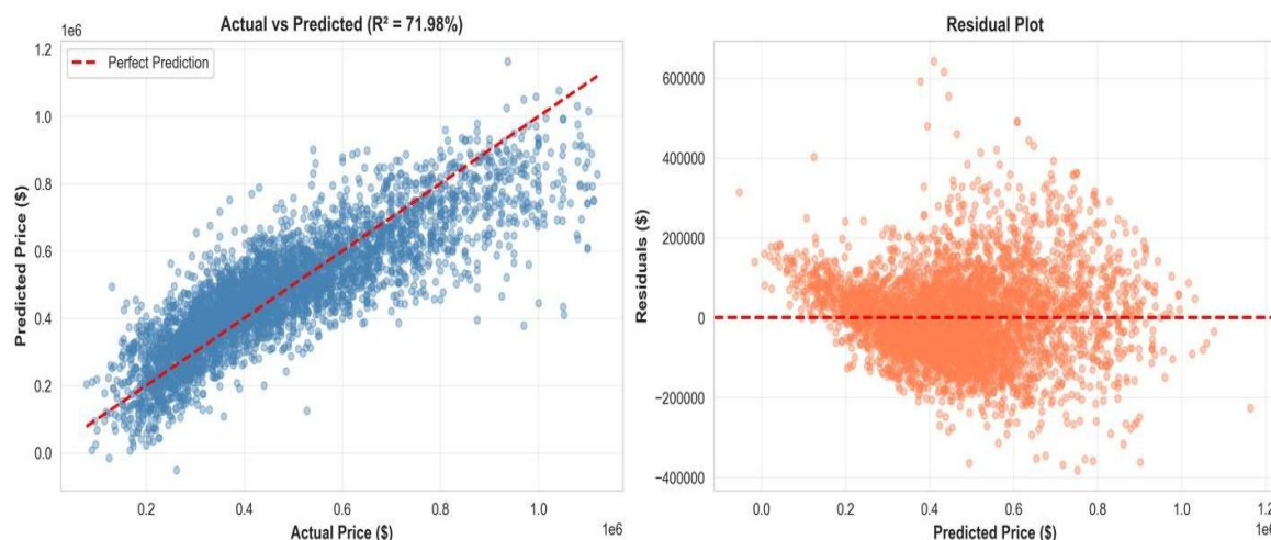
Fig. 4: Scatter plot of predicted versus actual prices showing strong linear correspondence with some heteroscedasticity at higher price ranges.
