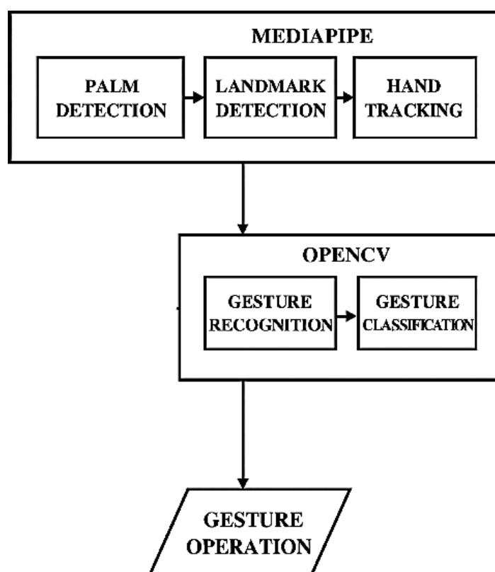
Fig. 3: Gesture operation flow.
