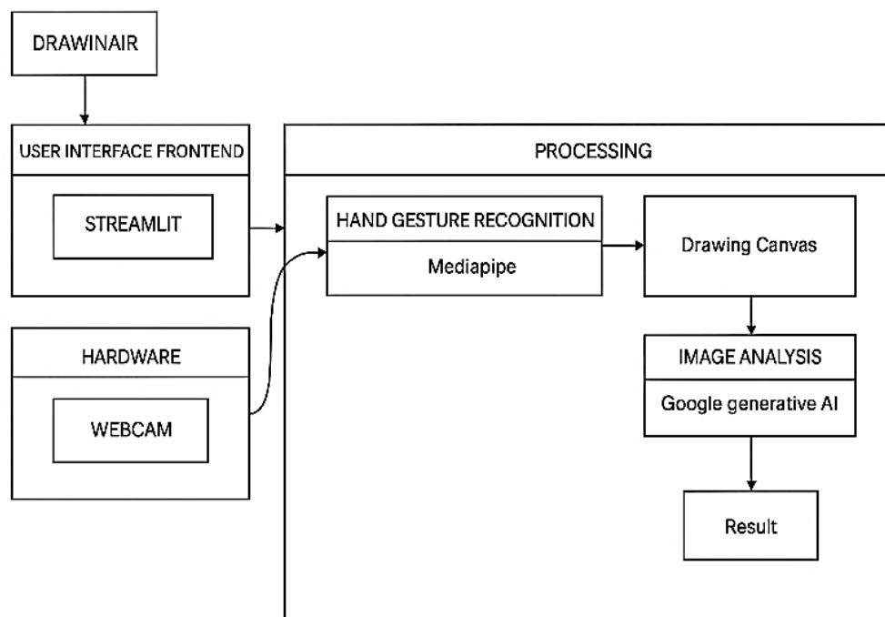
Fig 1: System architecture of the DrawInAir framework.
