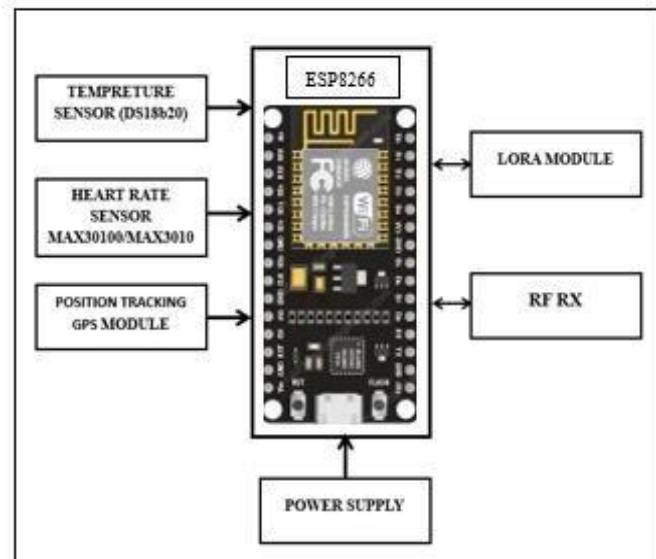
Fig. 1: Block diagram of transmitter (soldier) node.
