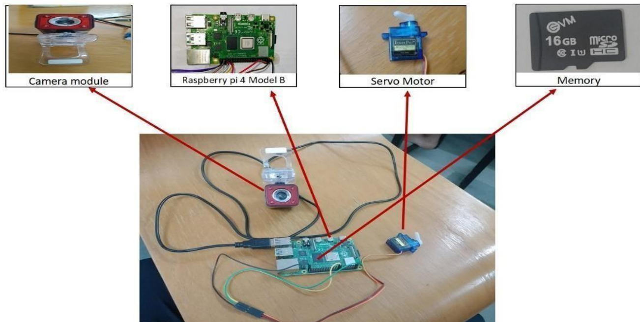
Fig. 4: Schematic representation of the proposed prototype.
