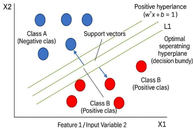
Fig. 2: Classification using SVM.
