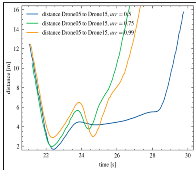
Fig. 8: The distance between the leader drones.
