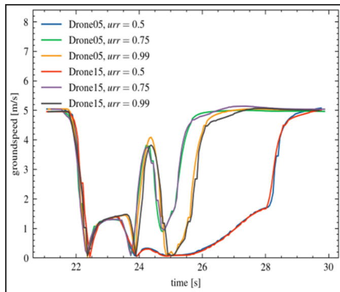
Fig. 7: The speed of the leader drones.
