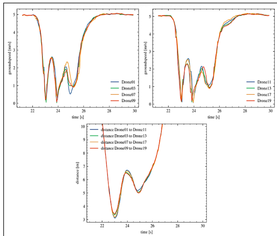
Fig. 6: The Speed Chart of selected Drones for both SWARMS (left and right charts) and the minimum distances (middle chart) for the parameter urr=0.75 .
