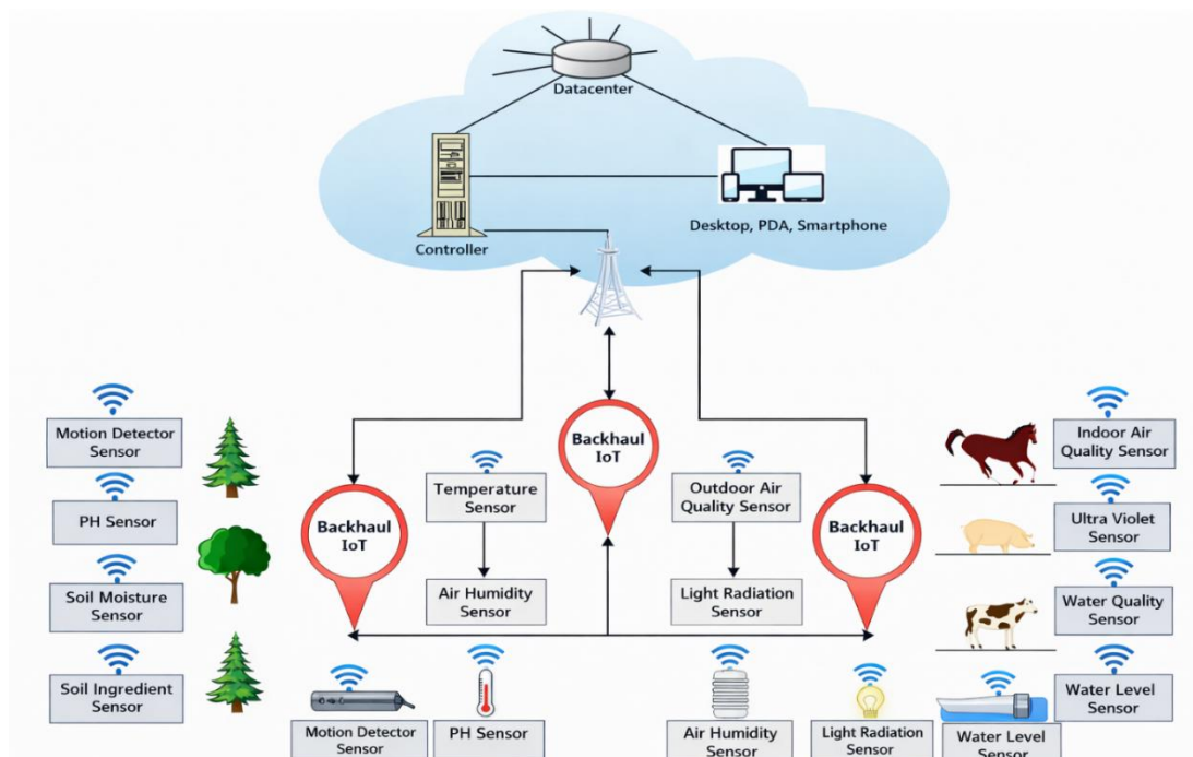
Fig. 4: IoT architecture for smart farming.
