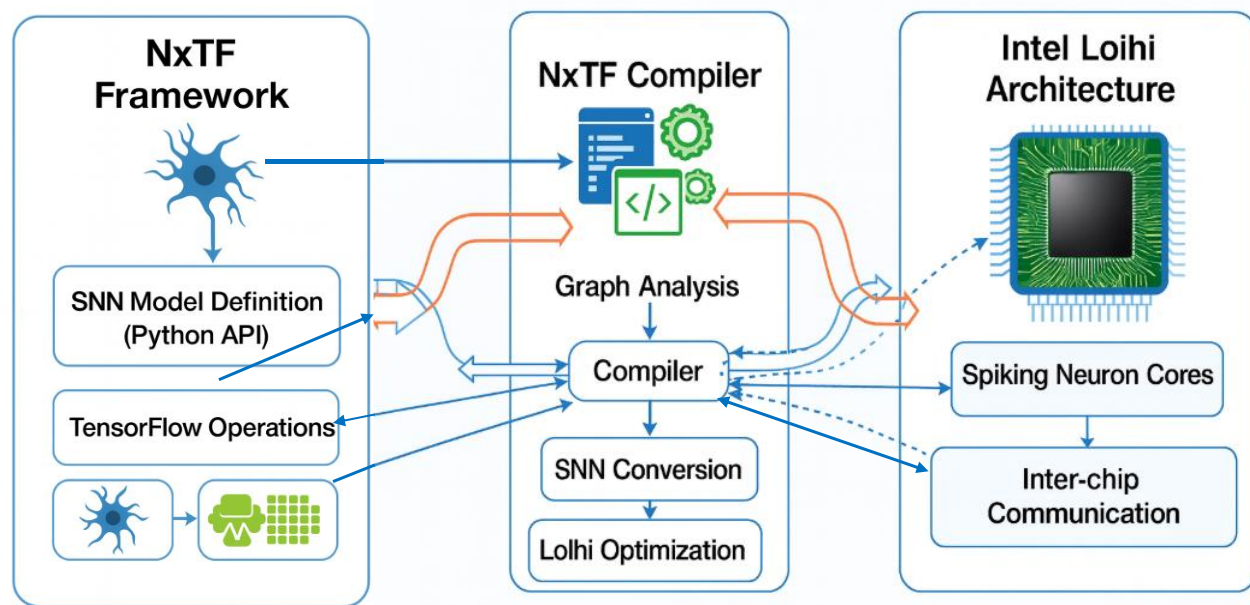
Fig. 2: Workflow integrating the NxTF framework with the Intel Loihi architecture.
