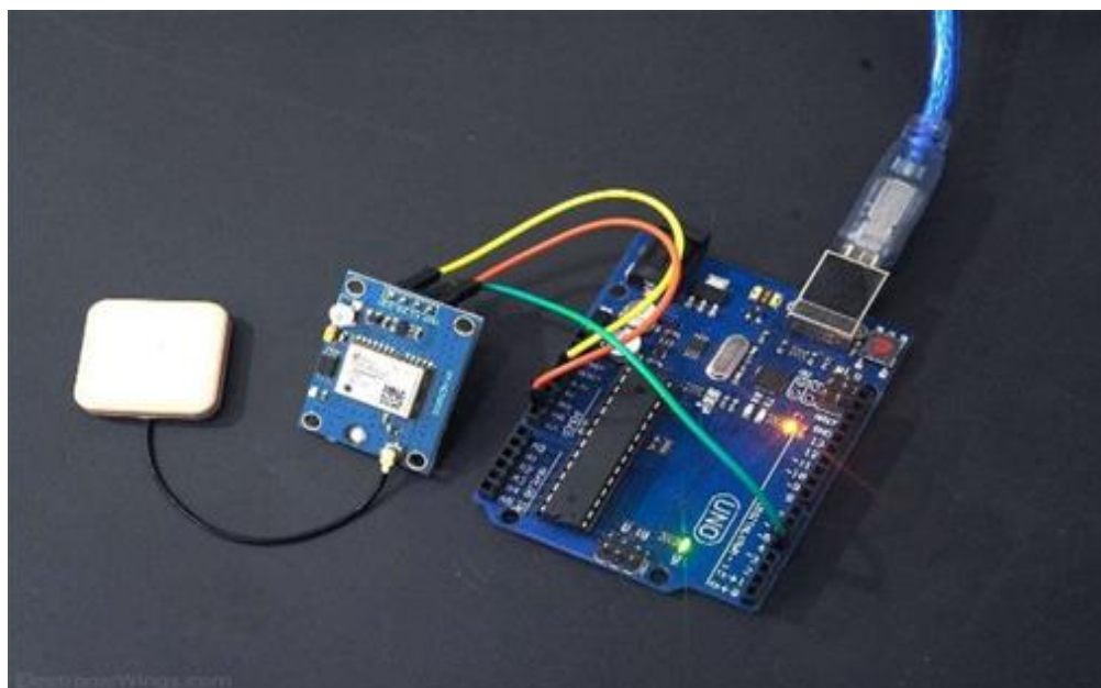
Fig. 8: GPS NEO-6M module connection with Arduino UNO for real-time position.
