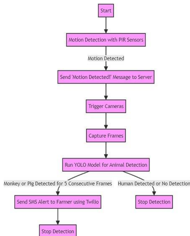
Fig. 1: Task network diagram.
