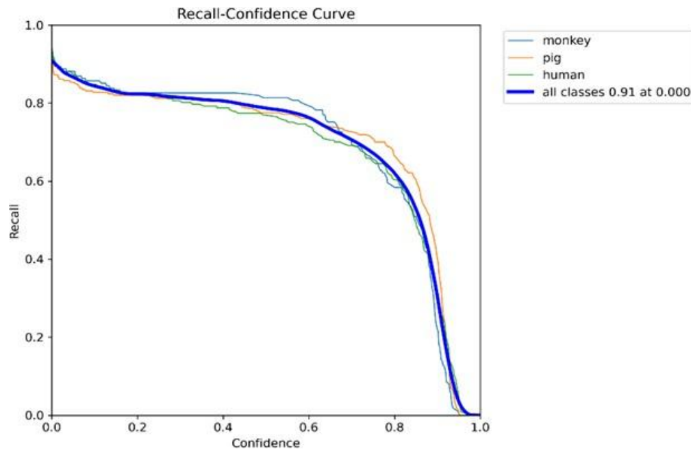
Fig. 9: Recall confidence curve.
