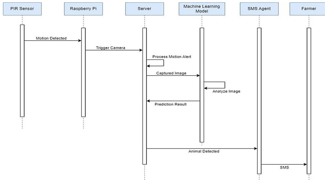
Fig. 2: Sequence diagram.
