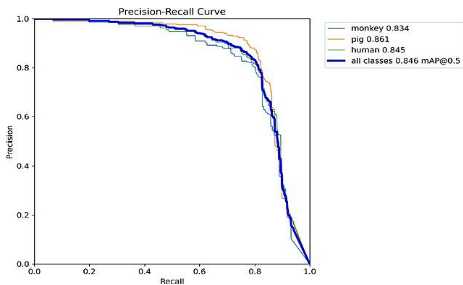
Fig. 7: Precision recall curve.
