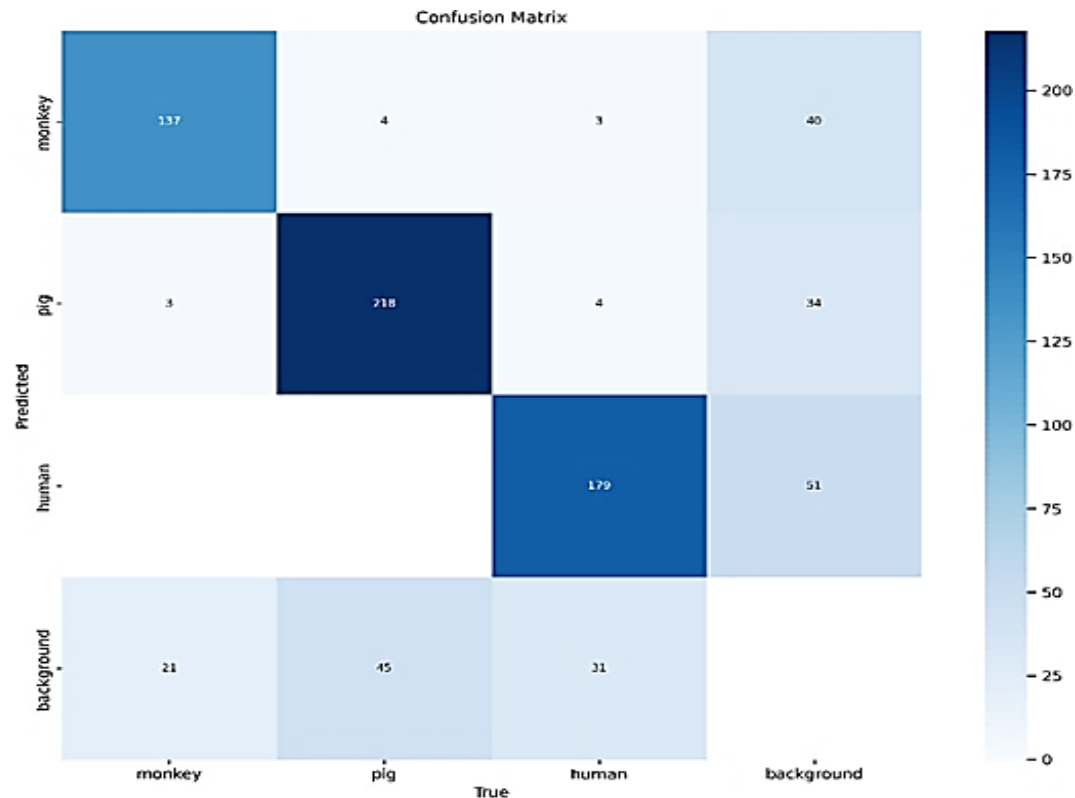
Fig. 5: Confusion matrix.
