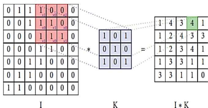
Fig. 7: 2D Convolution level function of a CNN.
