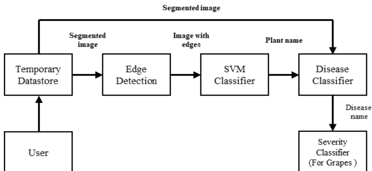
Fig. 5: Flow diagram of plant leaf disease classification mechanism.
