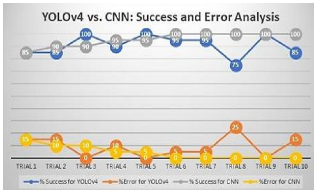
Fig. 16: Results of YOLOv4 vs CNN.
