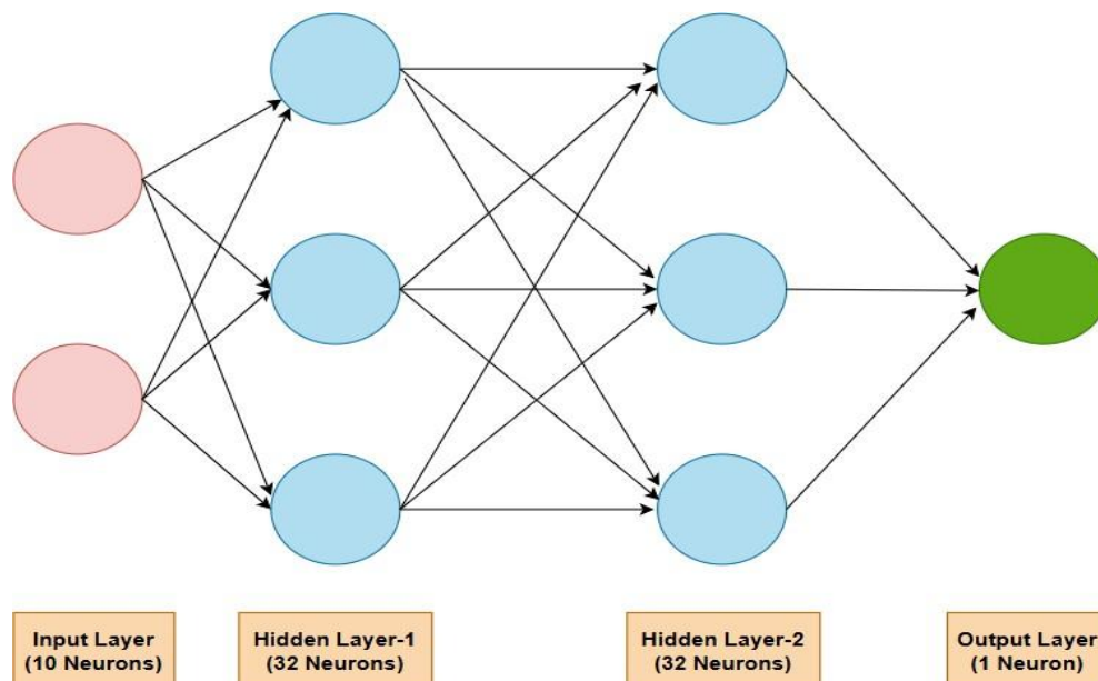
Fig. 2: Proposed 4-layer of ANN architecture.
