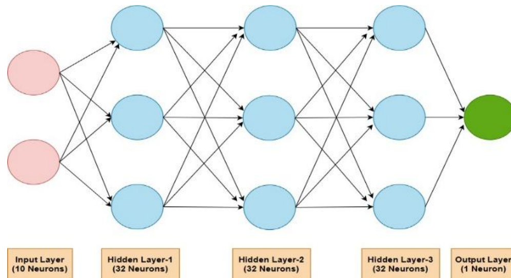
Fig. 3: Proposed 5-layer of ANN architecture.
