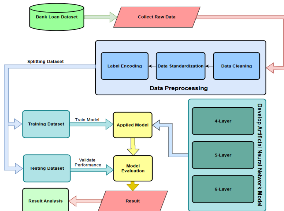
Fig. 1: Flow chart of proposed diagram.
