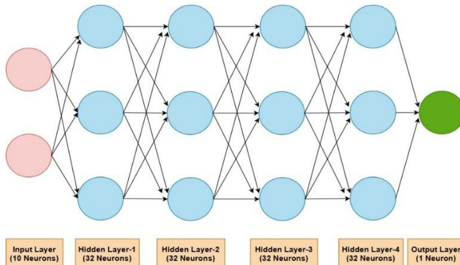
Fig. 4: Proposed 6-layer of ANN architecture.
