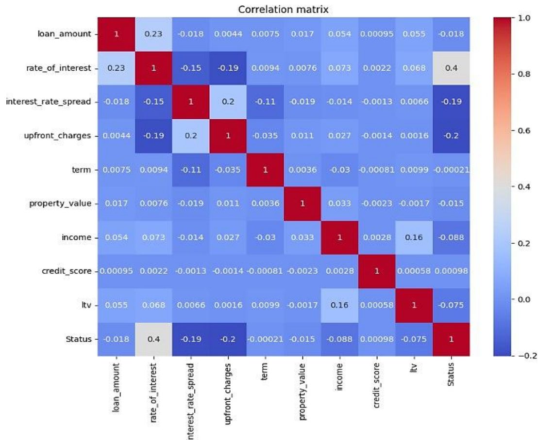
Fig. 6: Co-relation between features.
