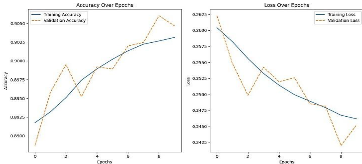
Fig. 5: Accuracy and loss curve.
