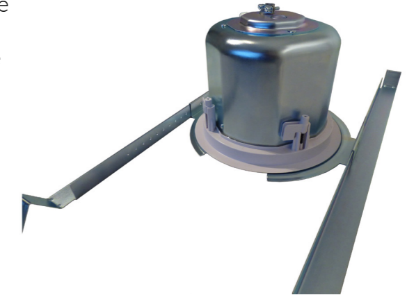
Figure 7.3: Loudspeaker positioning
