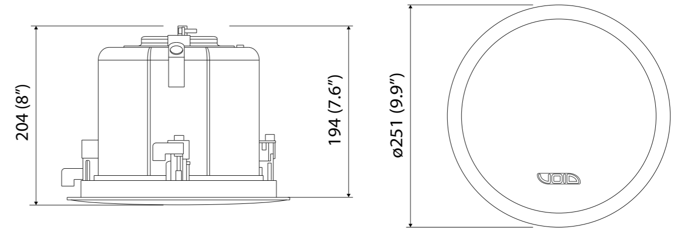
Figure 5.2: Cirrus 6.1 dimensions
