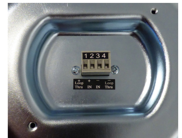
Figure 7.5: Terminal layout
