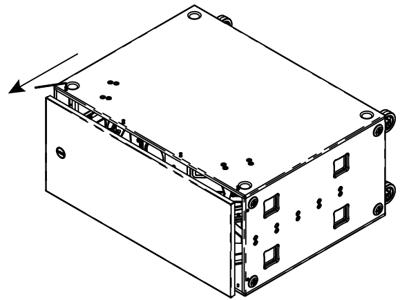
Figure 6.5: Grille removal
